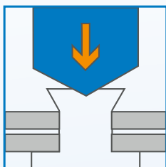
CAULKING
