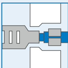
CRIMPING
